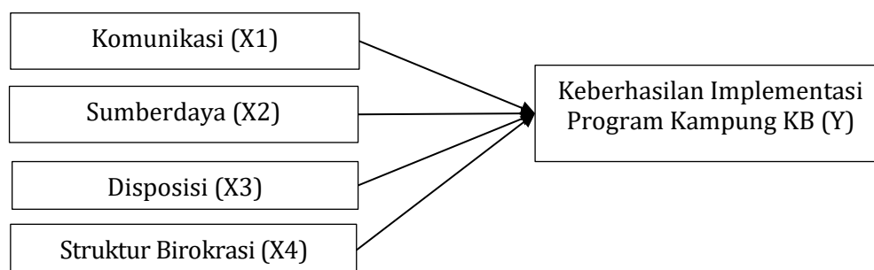
Gambar 2. Hipotesis Model Geometri
