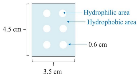
Figure 1. The finished paper device
