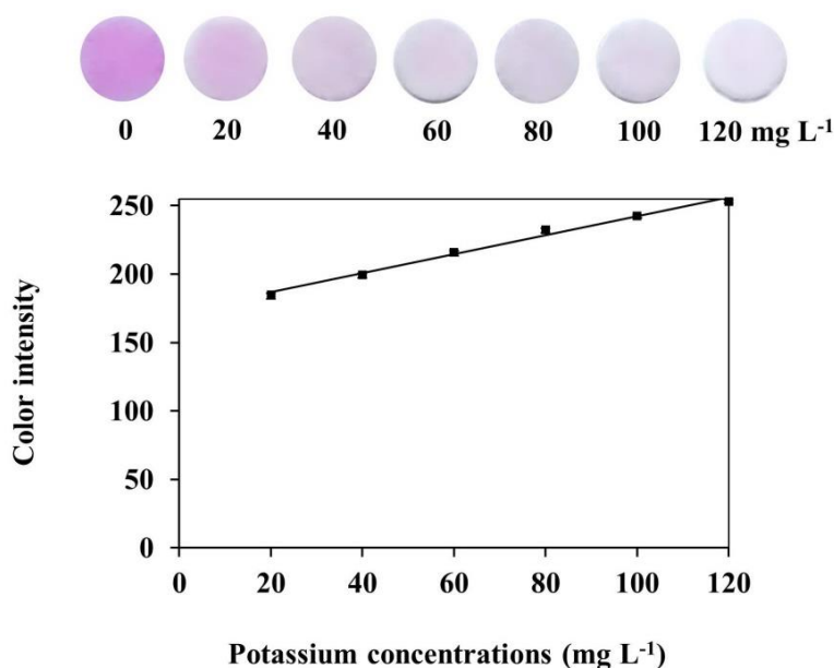
Figure 6. Images of color intensity of remaining calmagite on paper device for various concentrations of potassium and calibration curve of potassium obtained from indirect colorimetric determination using a paper device and smartphone
