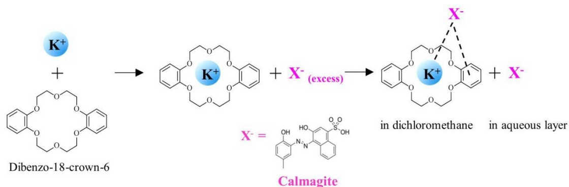
Figure 3. Schematic diagram to show the mechanism for ion-pair extraction of potassium
