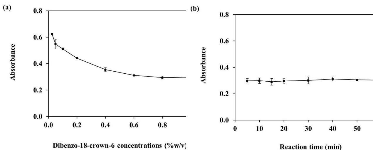
Figure 4. The effect of (a) dibenzo-18-crown-6 concentration and (b) reaction time on the ion-pair extraction
