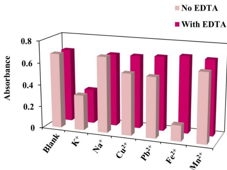
Figure 5. The effect of \text{K}^+ and other interference ions, compared with the blank, during extraction, with and without EDTA
