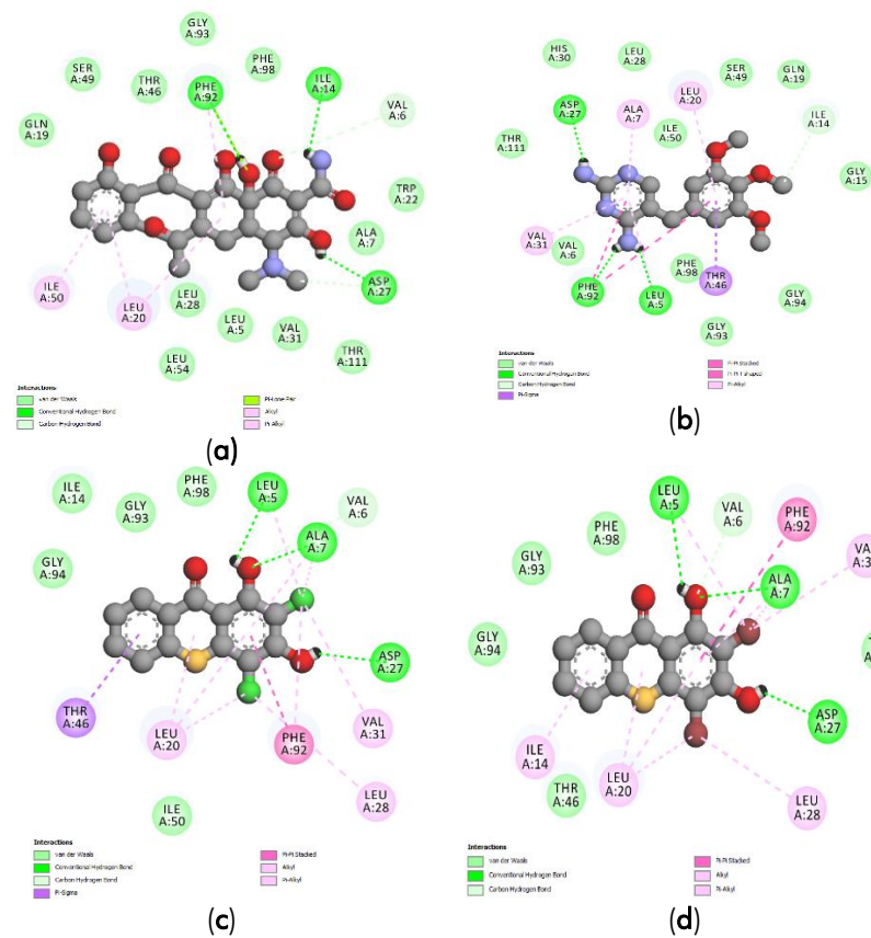
Figure 4. The interactions (a) tetracycline, (b) trimethoprim, (c) compound TX3, and (d) compound TX6 towards DHFR S. aureus protein
