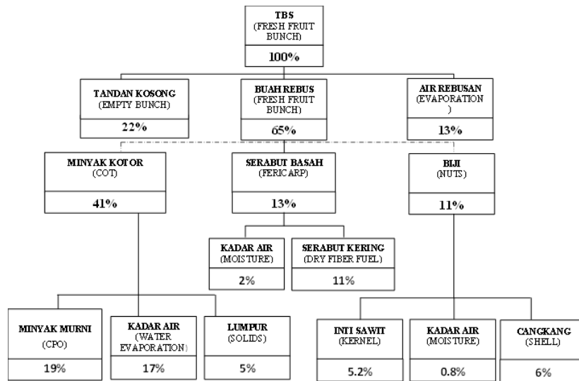
Gambar 5. Diagram material balance PT X
