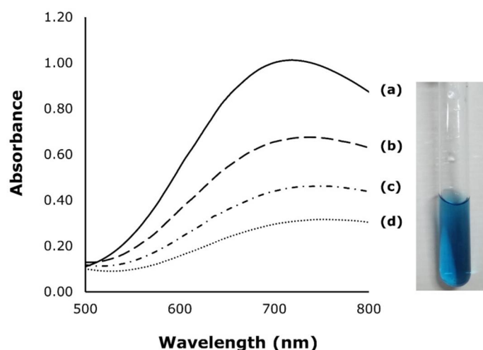
Figure 1. Visible spectrophotometric spectrum profile of formed Prussian blue and their solution colour. (a) Prussian blue without the addition of chlorine. Prussian blue with the addition of (b) 1.12 \text{ mmol L}^{-1} , (c) 2.8 \text{ mmol L}^{-1} , and (d) 11.2 \text{ mmol L}^{-1} of chlorine. Conditions were 2.0 \text{ mmol L}^{-1} ferrousulfate, 2.5 \text{ mmol L}^{-1} potassium ferricyanide, and 2.0 \text{ mol L}^{-1} hydrochloric acid with an incubation time of 1 min.
